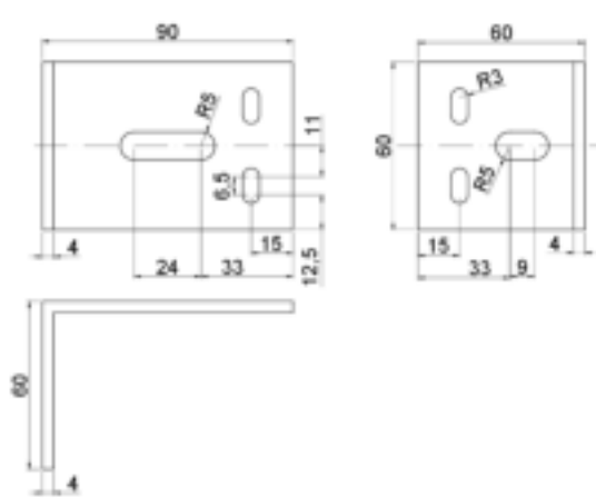
Figure 2.4d: CAA_60 x 90 x 60 x 4,0.
