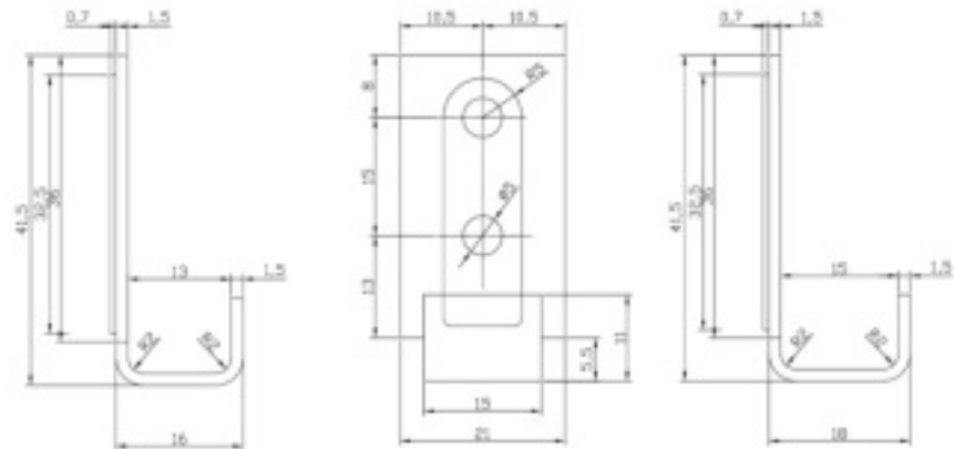
Figure A1.2b: CF-41,5x15x11 clip.
