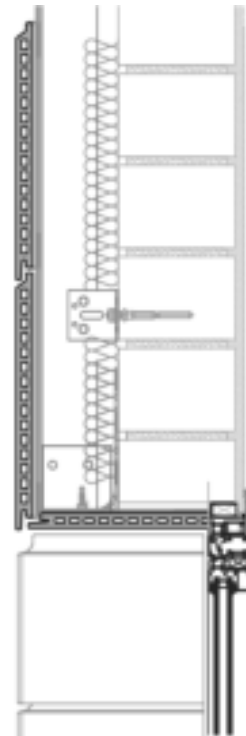
Figure A2.7c: Lintel with ceramic piece.
