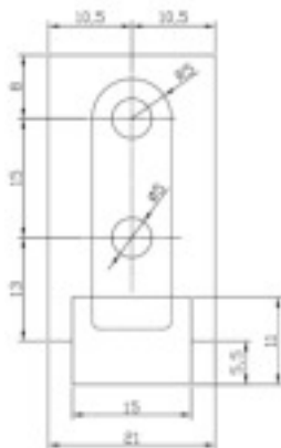
Figure A1.2a: CF-41,5x13x11 clip.
