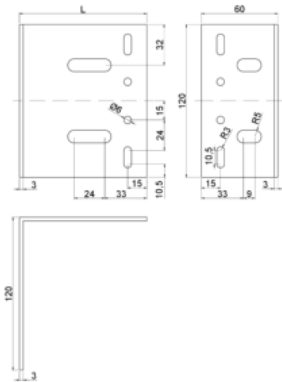
Figure 2.4a: CAA_120 x L x 60 x 3,0.
