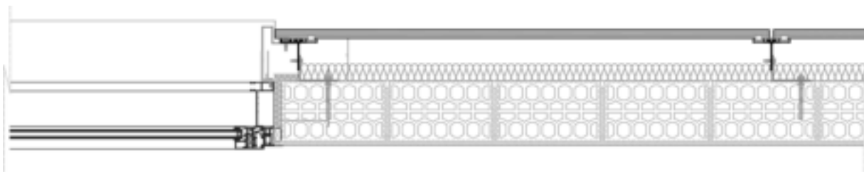
Figure A2.6b: Jamb with metal piece and blind.
