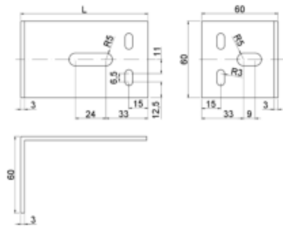
Figure 2.4c: CAA_60 x L x 60 x 3,0.
