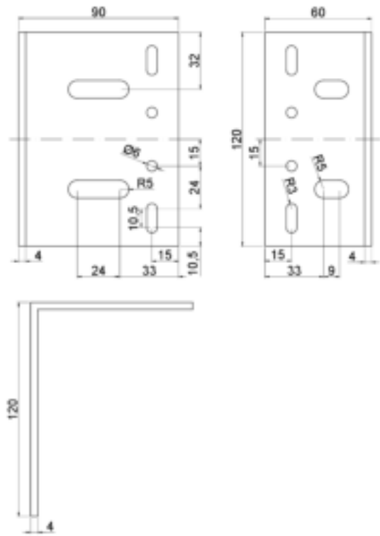
Figure 2.4b: CAA_120 x 90 x 60 x 4,0.
